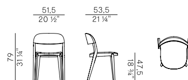
949/I sedia dining \ dining chair
