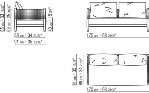
COD. 0295M7 CUSHION
