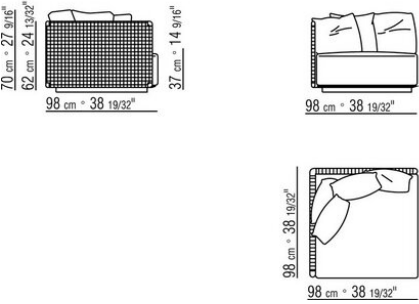
COD. 0265B1 END UNIT L
