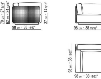
COD. 0265F1 ARMCHAIR WITHOUT ARMRESTS
