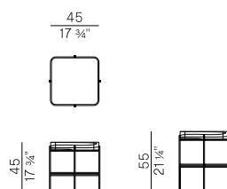
872/TQ tavolino \ coffee table
