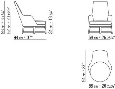
COD. 015M42 SOFT-ARMCHAIR METAL BASE W/MOV
