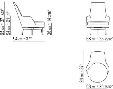
COD. 015M13 GA.13-ARMCHAIR WOODEN BASE
