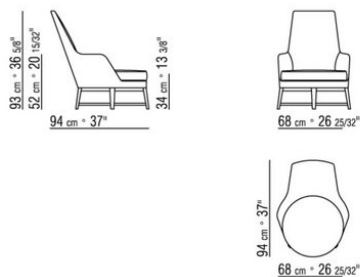
COD. 015M12 GA.12-ARMCHAIR METAL BASE W/MOV.
