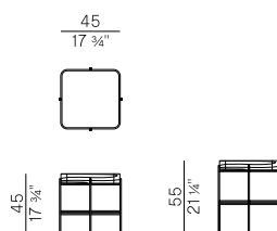
872/TQ tavolino \ coffee table
