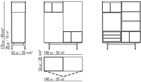
COD. 025470 CABINET
