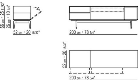
COD. 025469 CABINET / GLASS MODULES+DRAWER
