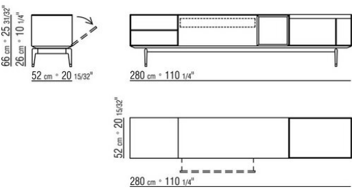
COD. 025470 CABINET
