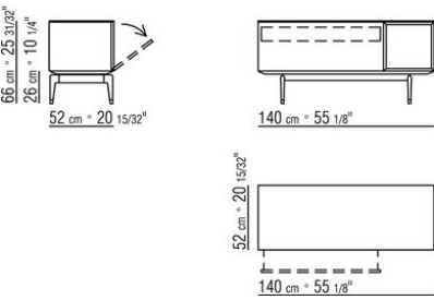
COD. 025463 CABINET / GLASS MODULES+DRAWER
