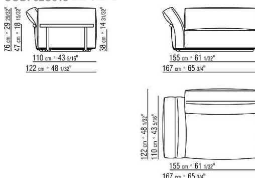
COD. 02C015 END UNIT L
