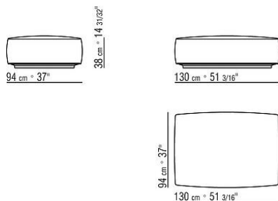
COD. 02C0G2 OTTOMAN
