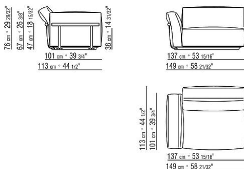
COD. 02C0C3 END UNIT L / LOW ARMREST
