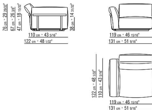
COD. 02C021 END UNIT L / LOW ARMREST
