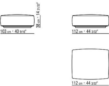
COD. 02C099 CUSHION
