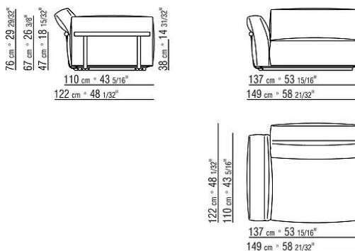
COD. 02C023 END UNIT L / LOW ARMREST
