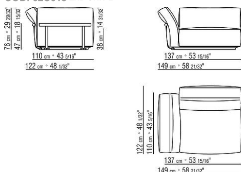
COD. 02C013 END UNIT L
