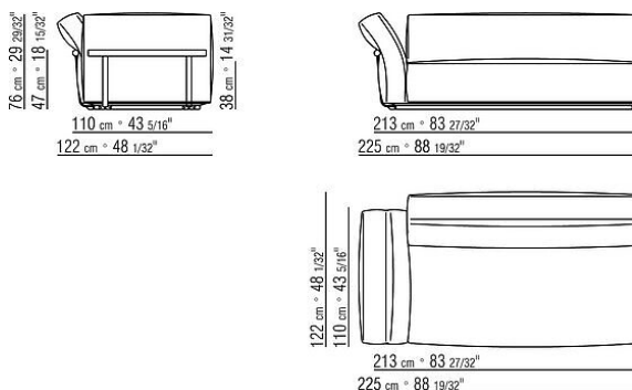
COD. 02C049 END UNIT L
