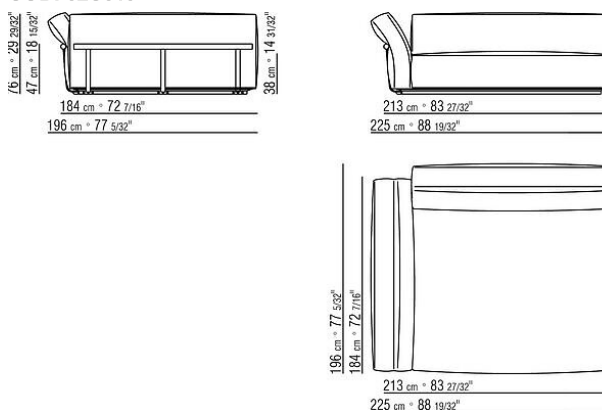
COD. 02C019 END UNIT L
