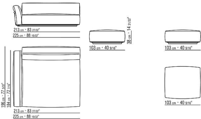
COD. 02C050 OTTOMAN
