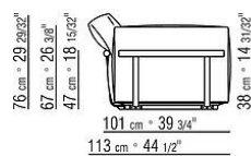
COD. 02C0C1 END UNIT L / LOW ARMREST
