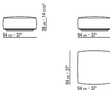
COD. 02C0G2 OTTOMAN
