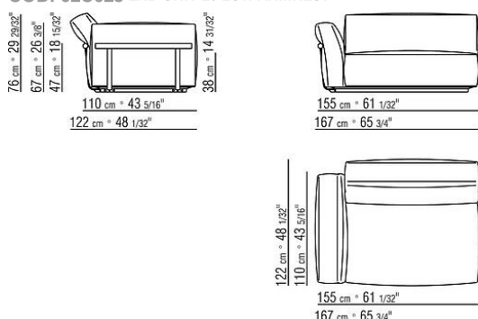
COD. 02C025 END UNIT L / LOW ARMREST
