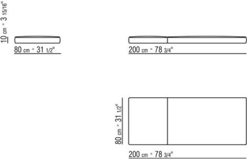
COD. 0273M9 SEAT / BACKREST CUSHION
