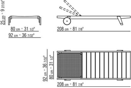
COD. 0273G2 DAYBED W/CASTORS
