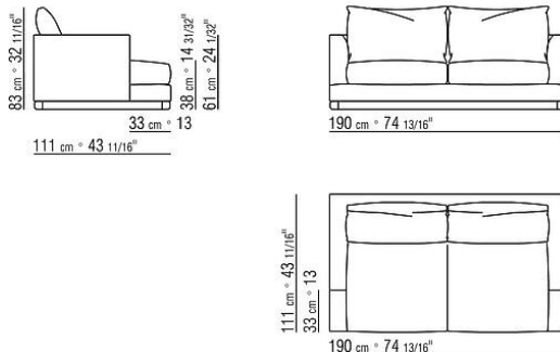
COD. 02D223 LONG ISLAND 24-END UNIT L
