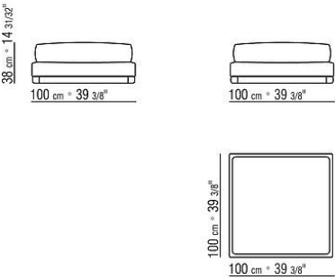
COD. 02D260 LONG ISLAND 24-OTTOMAN / DACRON
