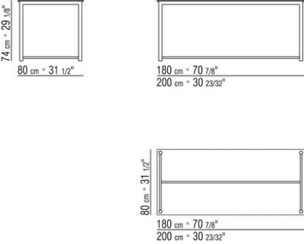
COD. 014550 TABLE GLASS TOP
