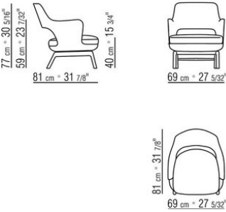
COD. 029625 ARMCHAIR SWIVEL BASE W/ 5 SPOKES
