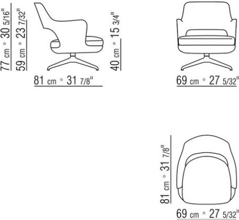
COD. 029624 ARMCHAIR SWIVEL BASE W/ 4 SPOKES
