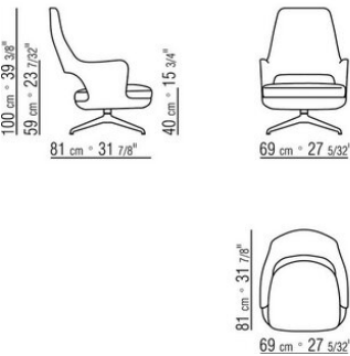
COD. 029634 BERGERE SWIVEL BASE W/ 4 SPOKES
