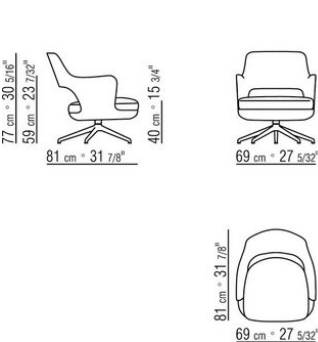
COD. 029625 ARMCHAIR SWIVEL BASE W/ 5 SPOKES
