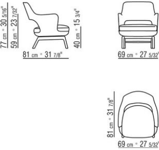
COD. 029624 ARMCHAIR SWIVEL BASE W/ 4 SPOKES
