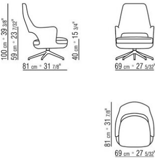
COD. 029635 BERGERE SWIVEL BASE W/ 5 SPOKES
