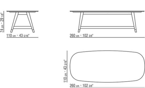
COD. 02A297 TABLE ASHWOOD BASE
