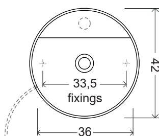
Pianta Top view
