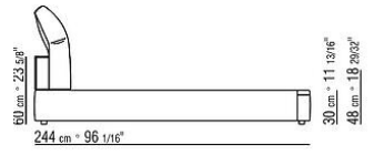
COD. 0243N5 SLIM BED W/STORAGE
