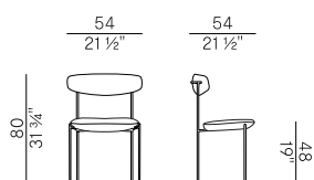
922 sedia dining \ dining chair
