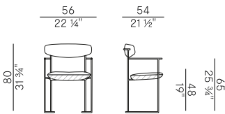
922/PMB poltroncina dining \ dining armchair
