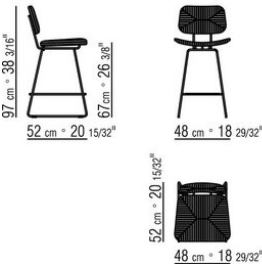
COD. 028068 S.H.-STOOL WITH BACK
