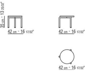
COD. 02A8K6 SMALL TABLE
