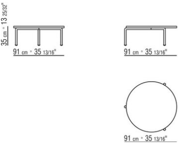
COD. 02A8K2 SMALL TABLE
