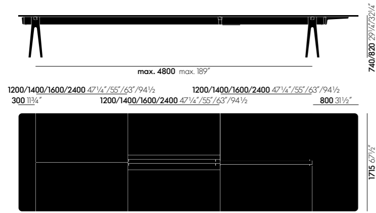
Joyn 2 Platform
