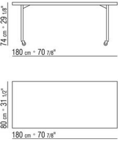
COD. 013093 "BEAN" TABLE W/CASTORS
